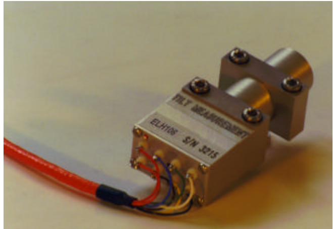
Type ELH106 High Precision Sensing Head for High vacuum use
